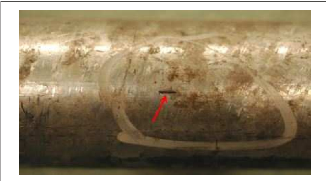
Fig. 14. Preferential grooving corrosion attack surrounding the weld seam area for a preaction system, near the pipe's 6 o'clock (bottom) installed position
